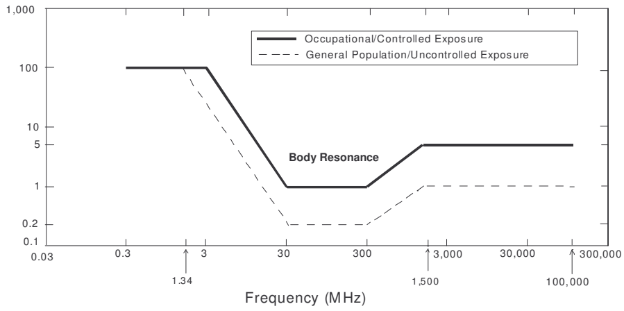
Figure 1. FCC Limits for Maximum Permissible Exposure (MPE) Plane-wave Equivalent Power Density
